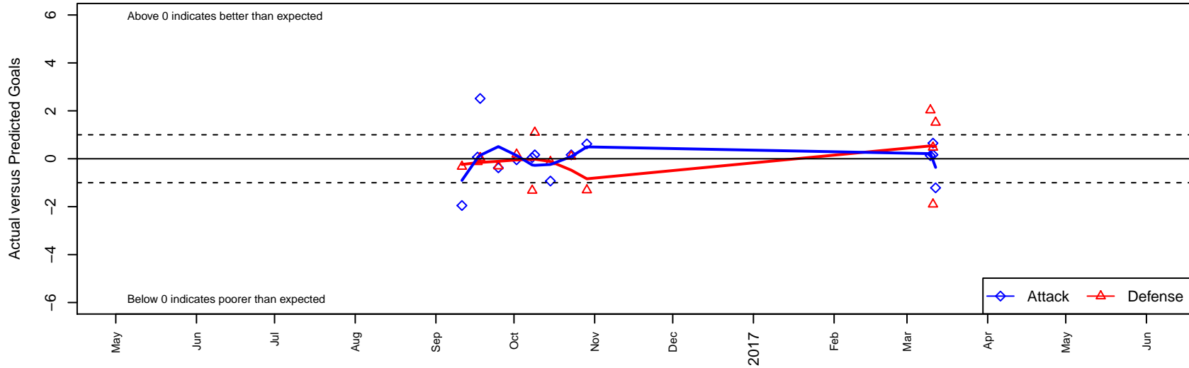
CDA Slammers HB C B98 Dots are actual minus expected GF (blue circles) and GA (red triangles). Blue line is smoothed change in attack strength. Red is smoothed change in defense strength.
